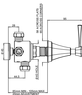
Concealed diverter 1 inlet 2 outlets with lever or crosstop handle with shut off
