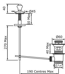
Combined pop-up waste and overflow with concealed pipes – 550mm
