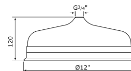
12" Easy clean shower rose
