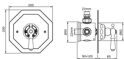
Concealed thermostatic shower mixer – secondary outlet connector
