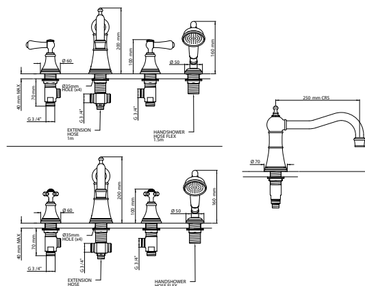
Three hole deck mounted bath filler with lever or crosstop handles
