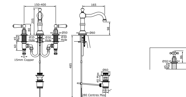
Three hole deck mounted basin mixer with high neck spout and lever or crosstop handles
