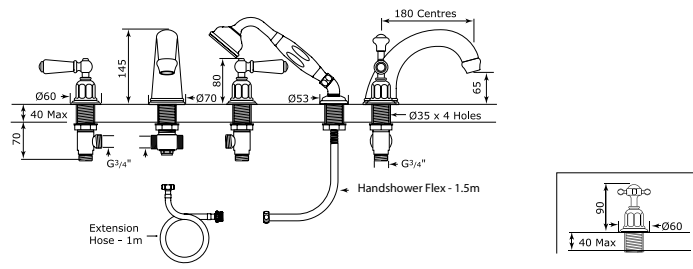
Three hole deck mounted bath filler with 255mm spout and lever or crosstop handles
