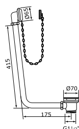
Combined pop-up waste and overflow with concealed pipes – 900mm
