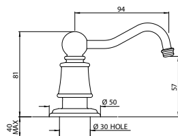
Single robe hook
