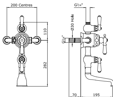
Exposed thermostatic bath shower mixer and deck unions with crosstop handles
