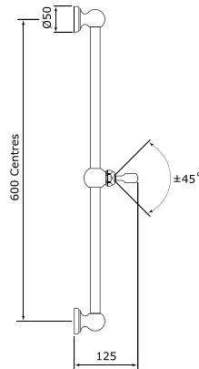
Sliding rail with shut off
