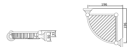
260mm bottle basket
