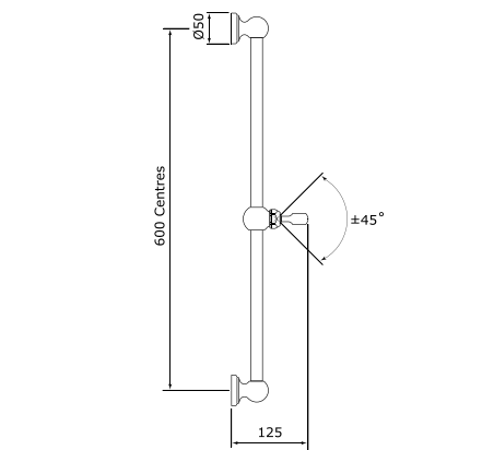
Sliding rail with shut off
