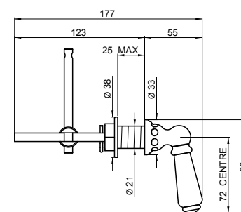
Extended Traditional concealed cistern lever
