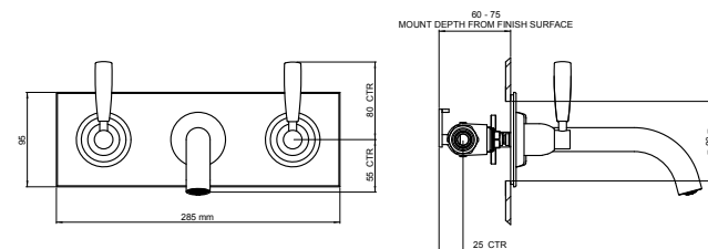
Three hole wall mounted basin mixer with lever handles
