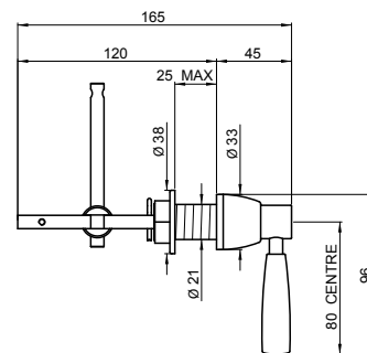
Extended Contemporary concealed cistern lever
