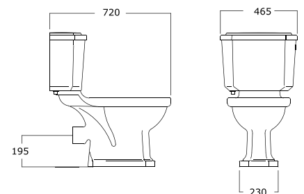
Four piece suite (Pan, Cistern, One/Two/Three Hole Basin and Pedestal)
