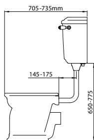
Low level WC (with flush mechanism)*
