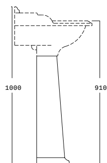
Basin – three hole
