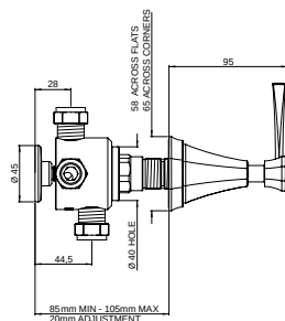
Concealed diverter 1 inlet 2 outlets with lever or crosstop handle with shut off
