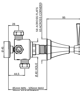
Concealed diverter 1 inlet 3 outlets with lever or crosstop handle
