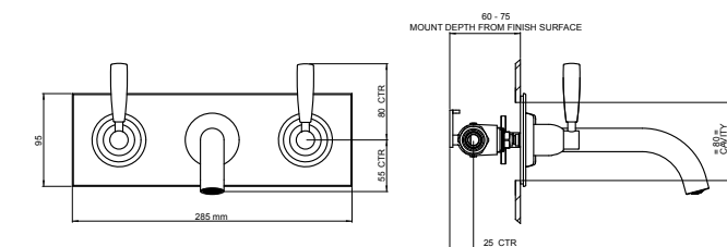
Three hole wall mounted basin mixer with lever handles
