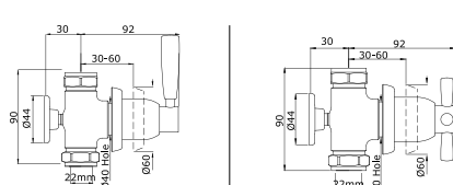
Single ½" wall valve
