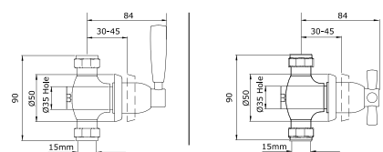
Concealed diverter with 1 inlet 2 outlets and lever or crosstop handle
