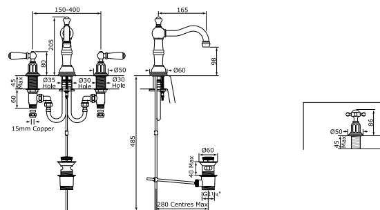
Three hole deck mounted basin mixer with high neck spout and lever or crosstop handles
