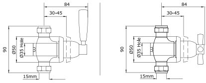
Concealed diverter with 1 inlet 2 outlets and lever or crosstop handle with shut off
