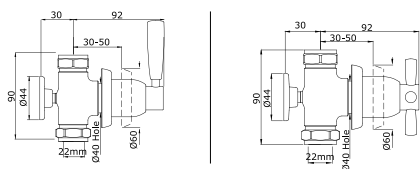
Pair ½" wall valves
