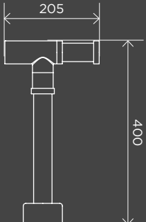
Round Bottle Trap for 32mm Basin Waste and 40mm Outlet
