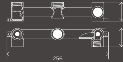
Concealed In-Wall Assembly for Bath and Basin Taps
