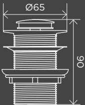
40mm Pop Up Waste - No Overflow / Unslotted
