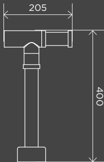
Round Bottle Trap for 32mm Basin Waste and 40mm Outlet MP05-R
