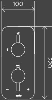
One-way Thermostatic Mixer Valve with Diverter
