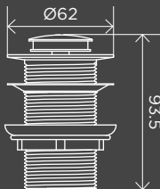
Basin Pop Up Waste 32mm - No Overflow / Unslotted MP04-B
