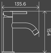
Piccola Basin Mixer Tap MB03XS
