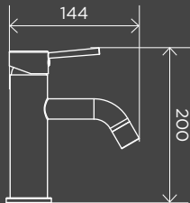
Round Basin Mixer Curved MB03
