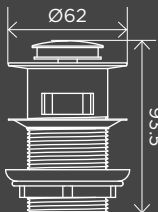
Basin Pop Up Waste 32mm - Overflow / Slotted MP04-A
