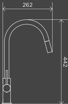
Piccola Pull Out Kitchen Mixer Tap MK17
