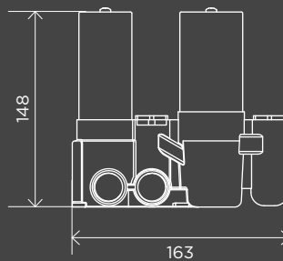
One-Way Thermostatic Shower Valve - Concealed Part
