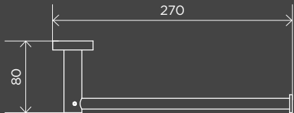
Round Guest Towel Rail MR05-R
