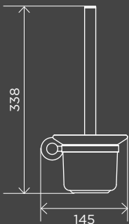
Round Toilet Brush and Holder MTO01-R
