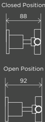
Cross Handle Jumper Valve Wall Top Assemblies MW08JL
