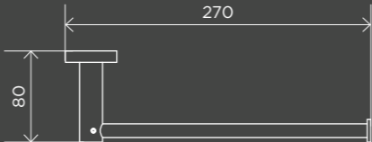
Round Guest Towel Rail
