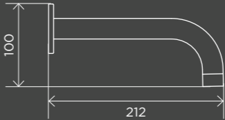
Round Curved Spout MS05
