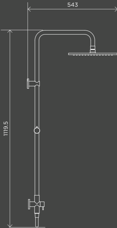
Round Combination Shower Rail 300mm Rose, Single-Function Hand Shower
