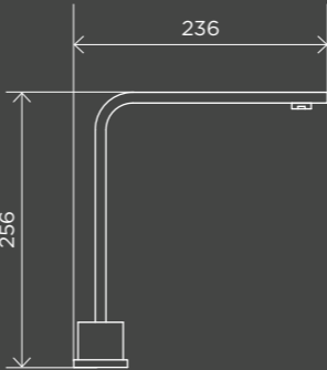
Square High-Rise Swivel Hob Spout MS09
