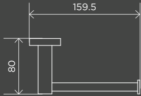
Square Toilet Roll Holder
