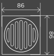
Square Floor Grate Shower Drain 80mm Outlet
