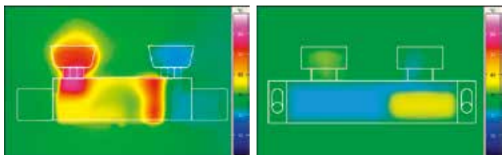
Thermal image without GROHE CoolTouch
