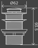
Basin Pop Up Waste 32mm - No Overflow / Unslotted MP04-B
