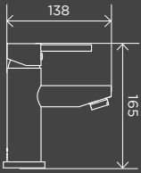
Round Basin Mixer MB02
