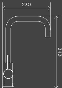
Round Kitchen Mixer Tap MK02
