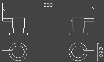
Round Quarter Turn Wall Top Assemblies MW06-SET
