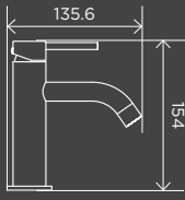
Piccola Basin Mixer Tap MB03XS
