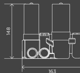
Two-Way Thermostatic Shower Valve - Concealed Part
