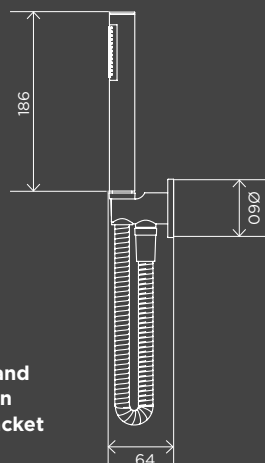
Pull Out Hand Shower for Bath
