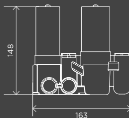
One-Way Thermostatic Shower Valve - Concealed Part
