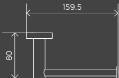
Round Toilet Roll Holder MR02-R
