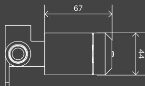
Concealed Body for Wall Mixers
