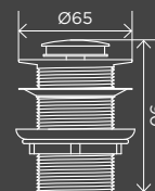
40mm Pop Up Waste - No Overflow / Unslotted
