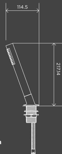
Pull Out Hand Shower for Bath
