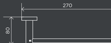
Round Guest Towel Rail
