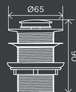
40mm Pop Up Waste - No Overflow / Unslotted
