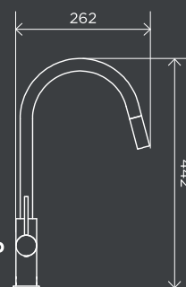
Piccola Pull Out Kitchen Mixer Tap
