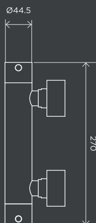
Exposed Thermostatic Shower Valve
