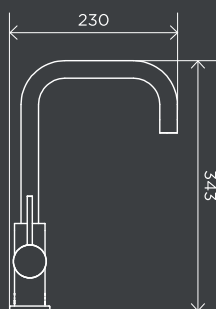
Round Kitchen Mixer Tap
