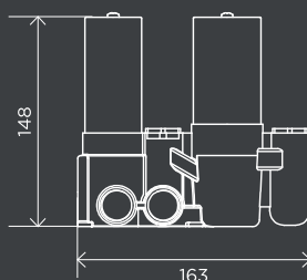
One-Way Thermostatic Shower Valve - Concealed Part
