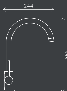
Piccola Pull Out Kitchen Mixer Tap
