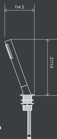
Pull Out Hand Shower for Bath
