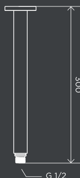
Round Ceiling Shower Arm 300mm
