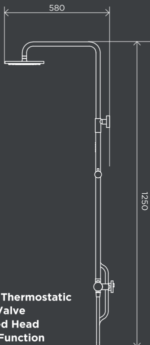
Exposed Thermostatic Shower Valve
